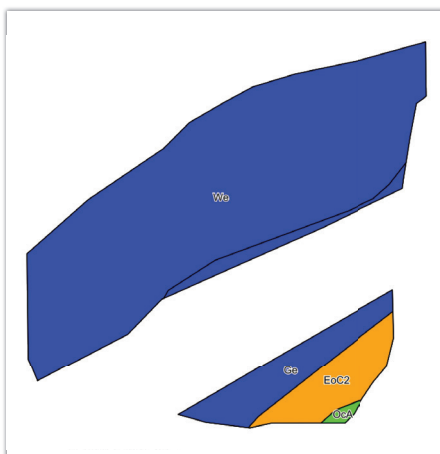
SOIL MAP
